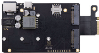
M2X Extension Ultra-thin version of this extension board
