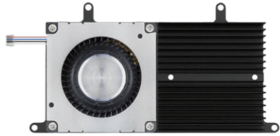
Edge2's Active Cooling Kit Edge Heatsink + 3705 Cooling Fan
